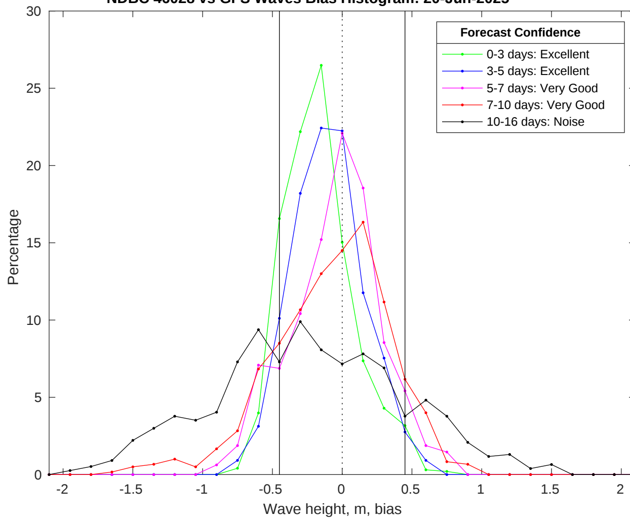
NDBC 46028 vs GFS Waves Bias Histogram: 20-Jun-2025
