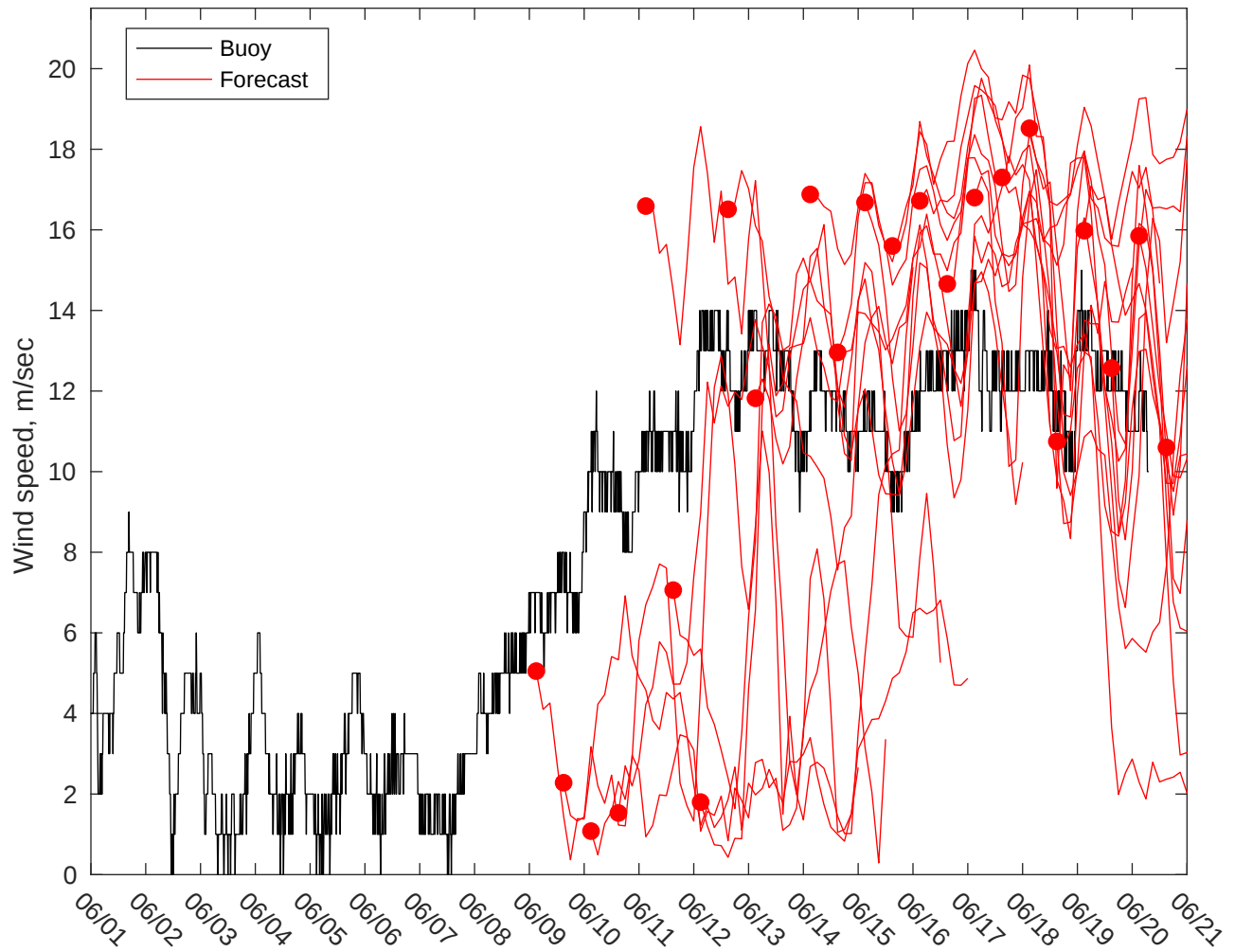
NDBC 46028 vs GFS Winds: 10 to 16 day forecast
