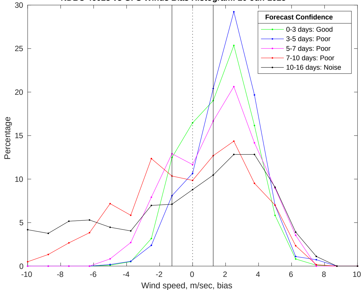
NDBC 46028 vs GFS Winds Bias Histogram: 20-Jun-2025
