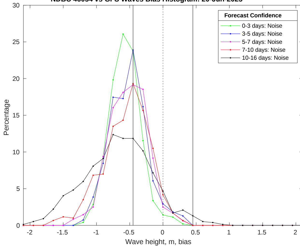
NDBC 46054 vs GFS Waves Bias Histogram: 20-Jun-2025
