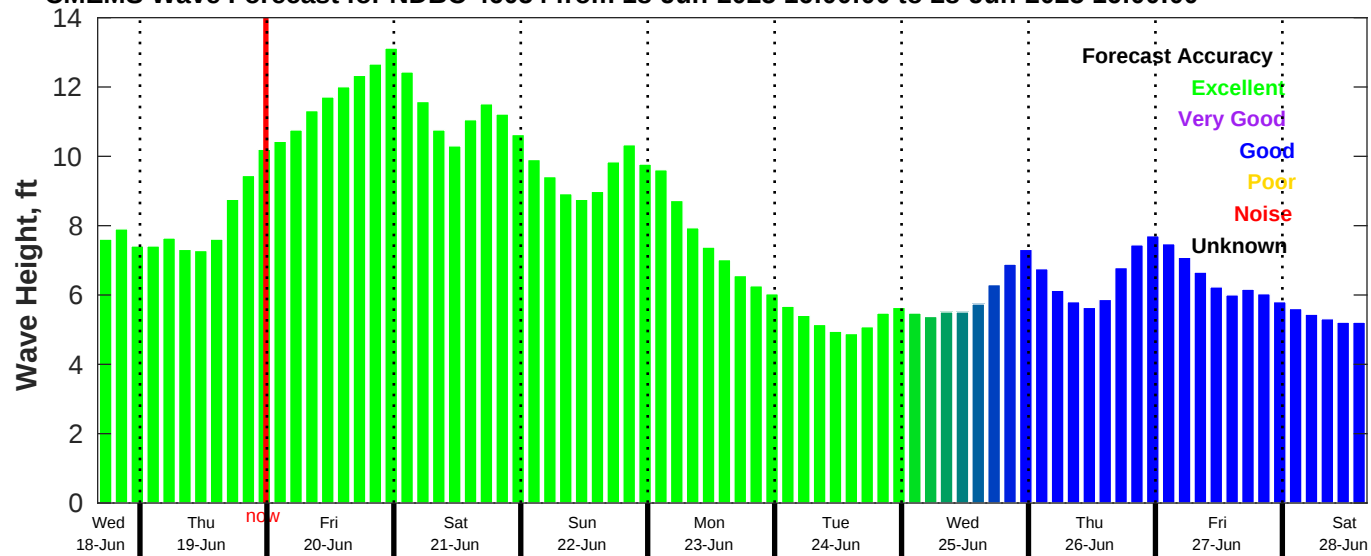
CMEMS Wave Forecast for NDBC 46054 from 18-Jun-2025 16:00:00 to 28-Jun-2025 16:00:00
