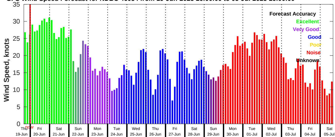
GFS Wind Speed Forecast for NDBC 46054 from 19-Jun-2025 16:00:00 to 05-Jul-2025 16:00:00
