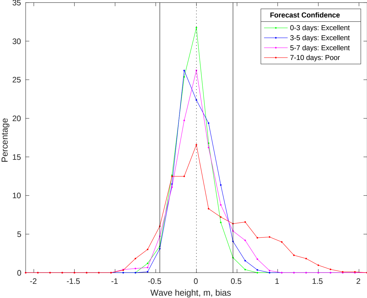
NDBC 46069 vs CMEMS Waves Bias Histogram: 20-Jun-2025
