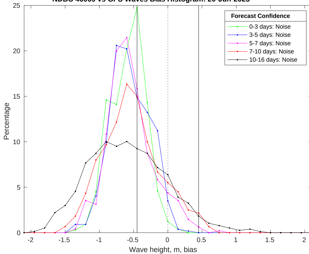
NDBC 46069 vs GFS Waves Bias Histogram: 20-Jun-2025
