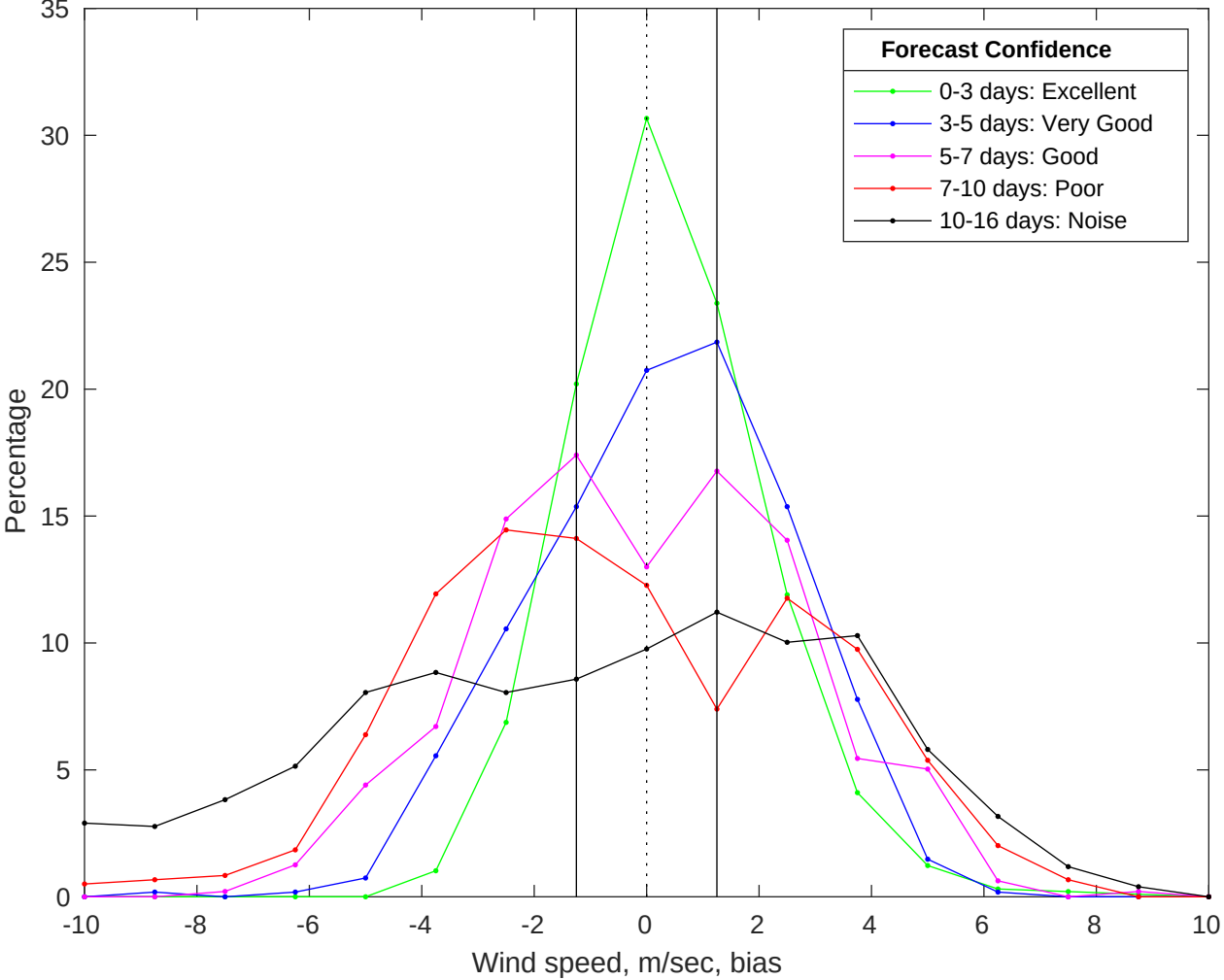
NDBC 46069 vs GFS Winds Bias Histogram: 20-Jun-2025
