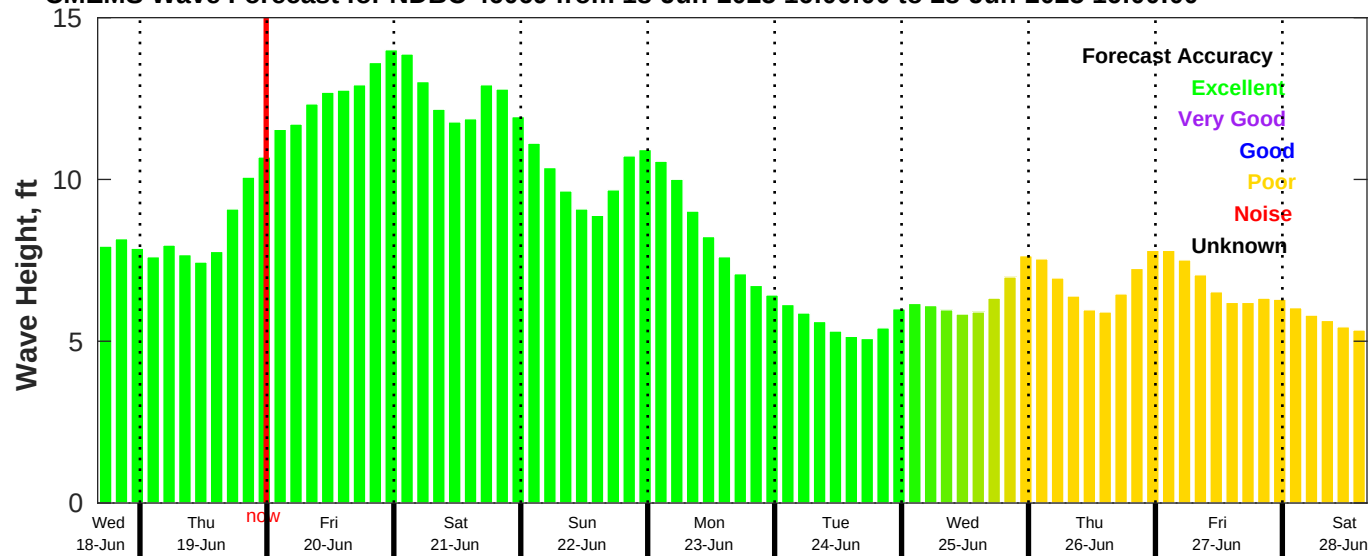
CMEMS Wave Forecast for NDBC 46069 from 18-Jun-2025 16:00:00 to 28-Jun-2025 16:00:00
