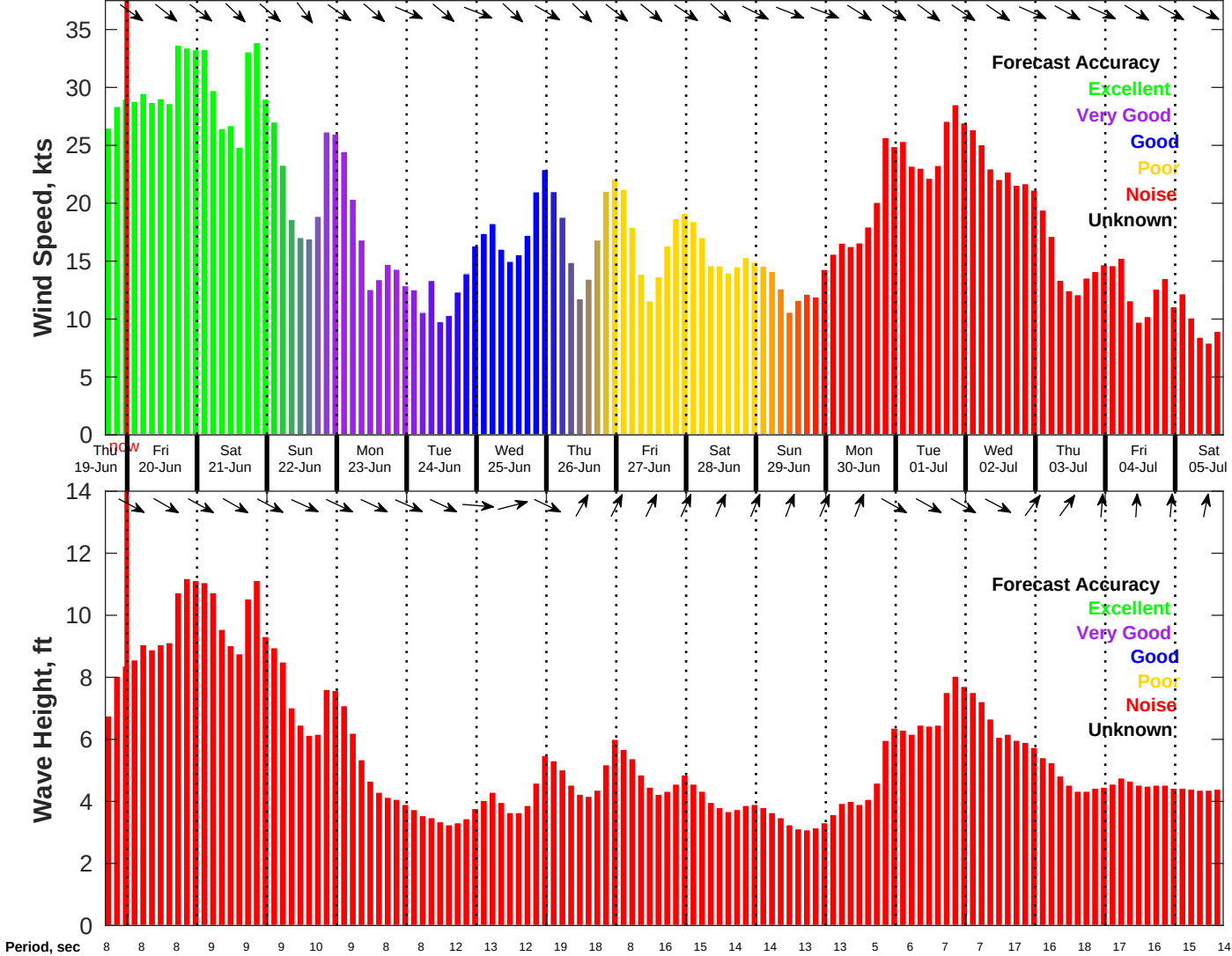
Wind & Wave Forecast for NDBC 46069 from 19-Jun-2025 16:00:00 to 05-Jul-2025 16:00:00
