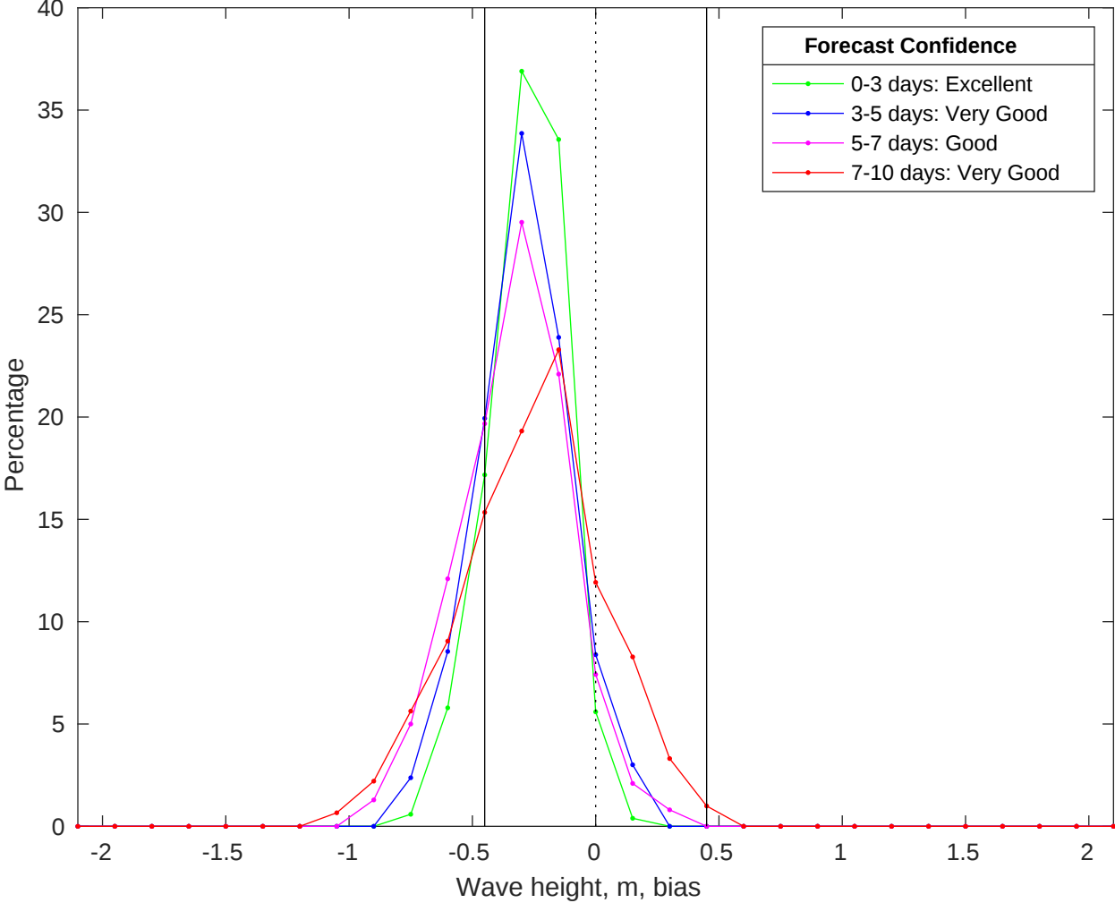
NDBC 51209 vs CMEMS Waves Bias Histogram: 20-Jun-2025
