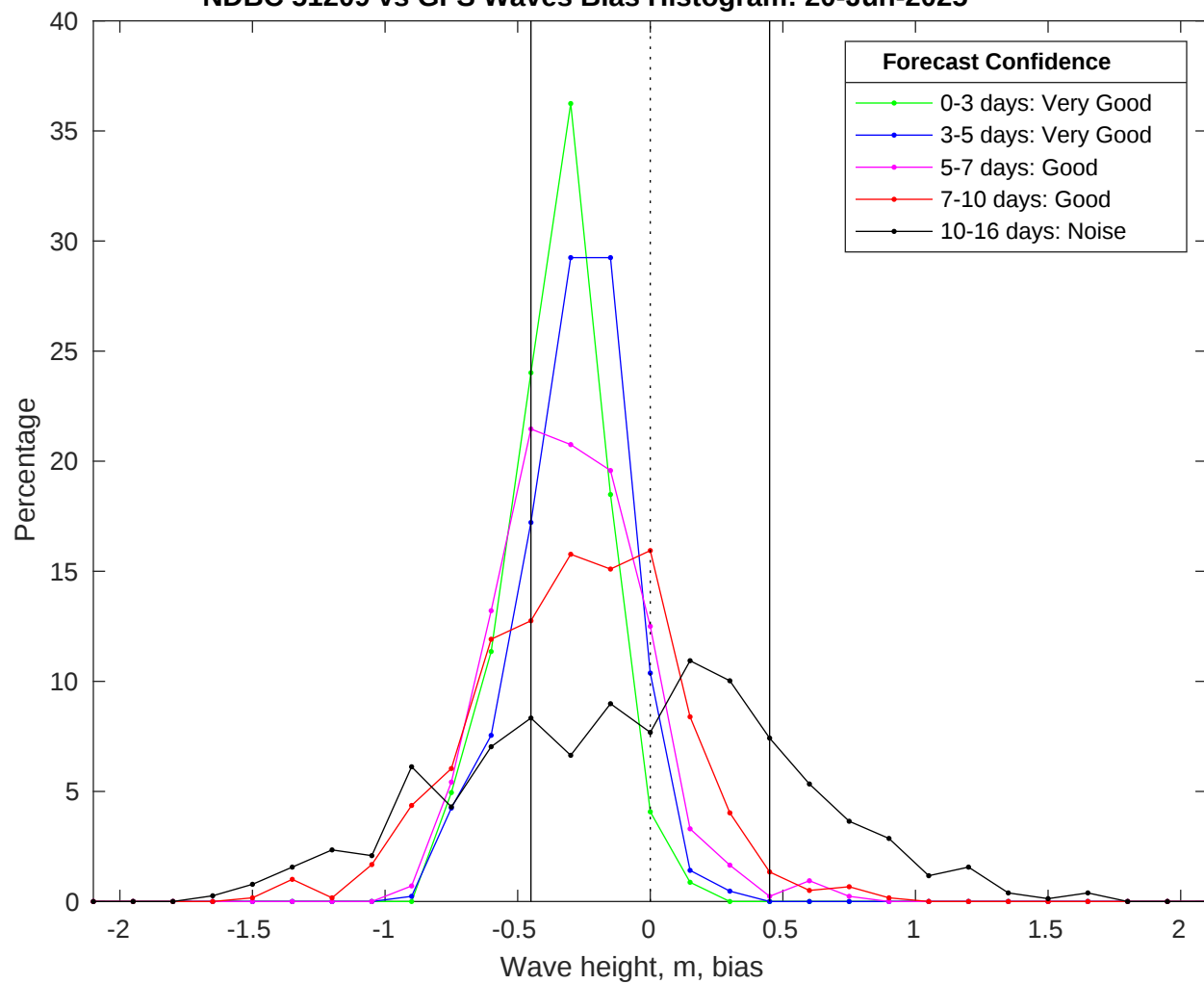
NDBC 51209 vs GFS Waves Bias Histogram: 20-Jun-2025
