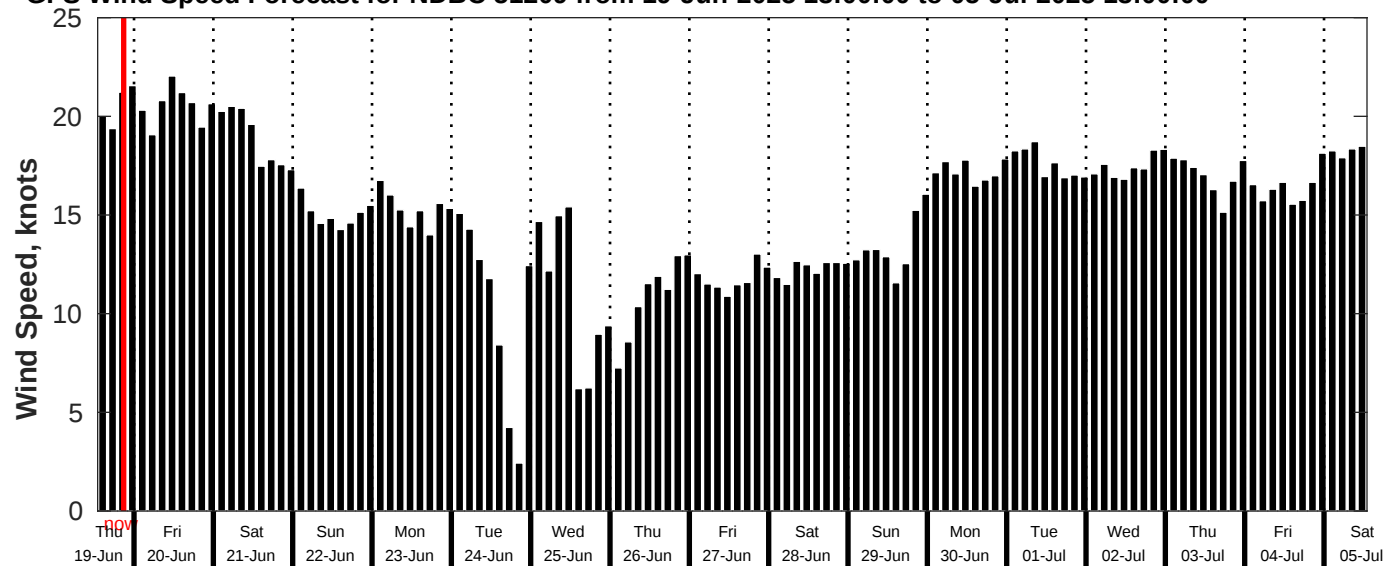
GFS Wind Speed Forecast for NDBC 51209 from 19-Jun-2025 13:00:00 to 05-Jul-2025 13:00:00
