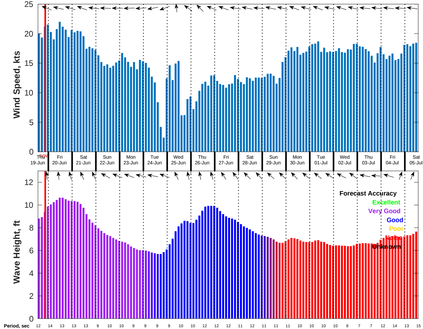
Wind & Wave Forecast for NDBC 51209 from 19-Jun-2025 13:00:00 to 05-Jul-2025 13:00:00
