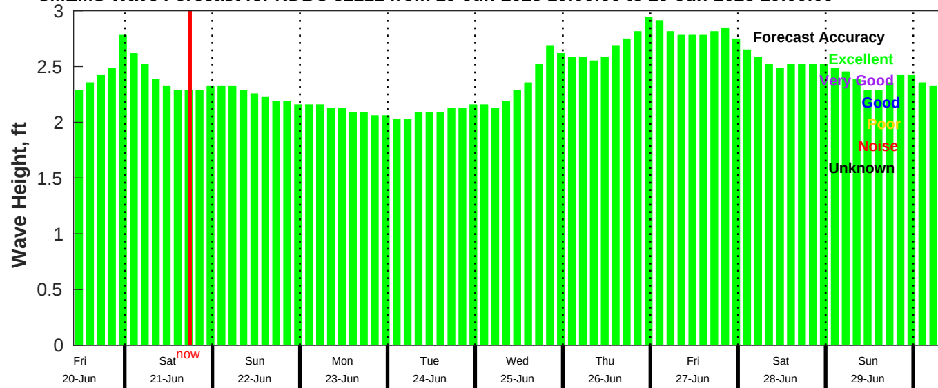
CMEMS Wave Forecast for NDBC 52211 from 19-Jun-2025 10:00:00 to 29-Jun-2025 10:00:00
