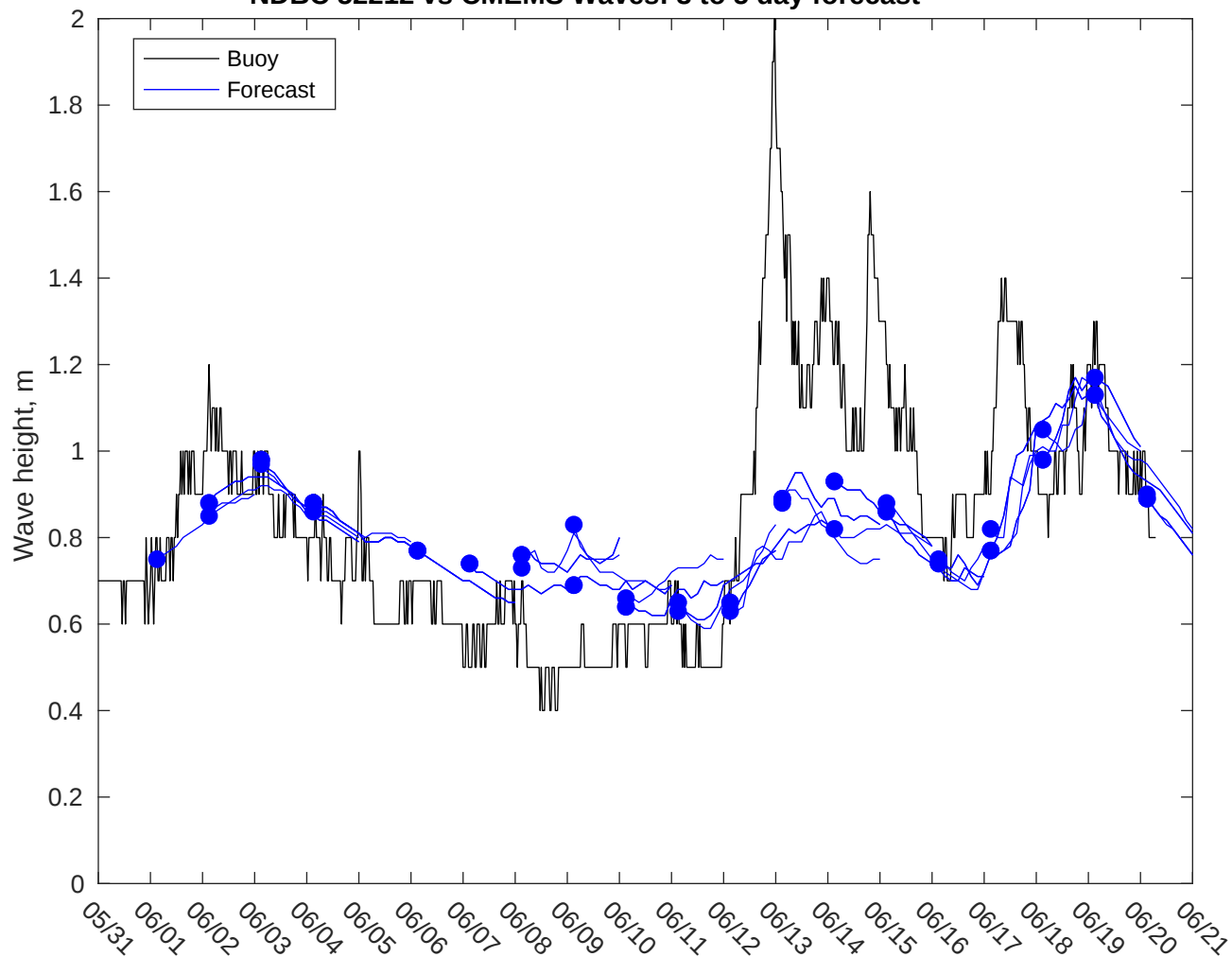
NDBC 52212 vs CMEMS Waves: 3 to 5 day forecast
