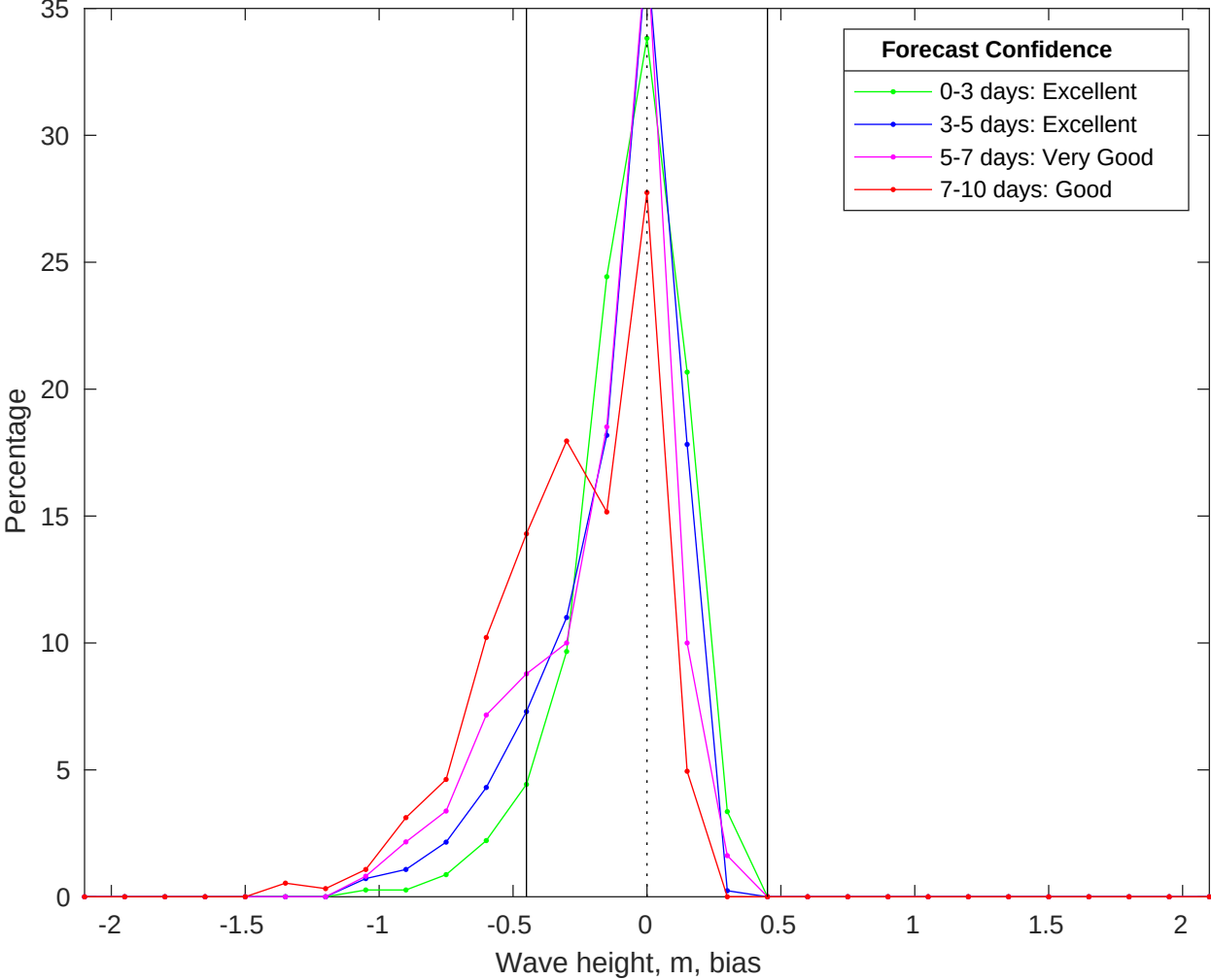
NDBC 52212 vs CMEMS Waves Bias Histogram: 20-Jun-2025
