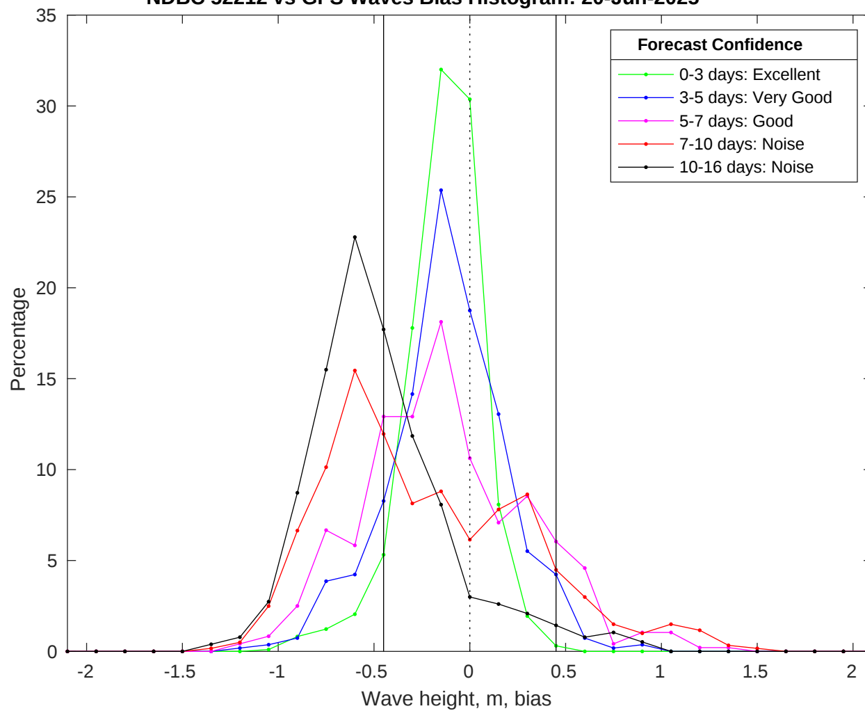
NDBC 52212 vs GFS Waves Bias Histogram: 20-Jun-2025
