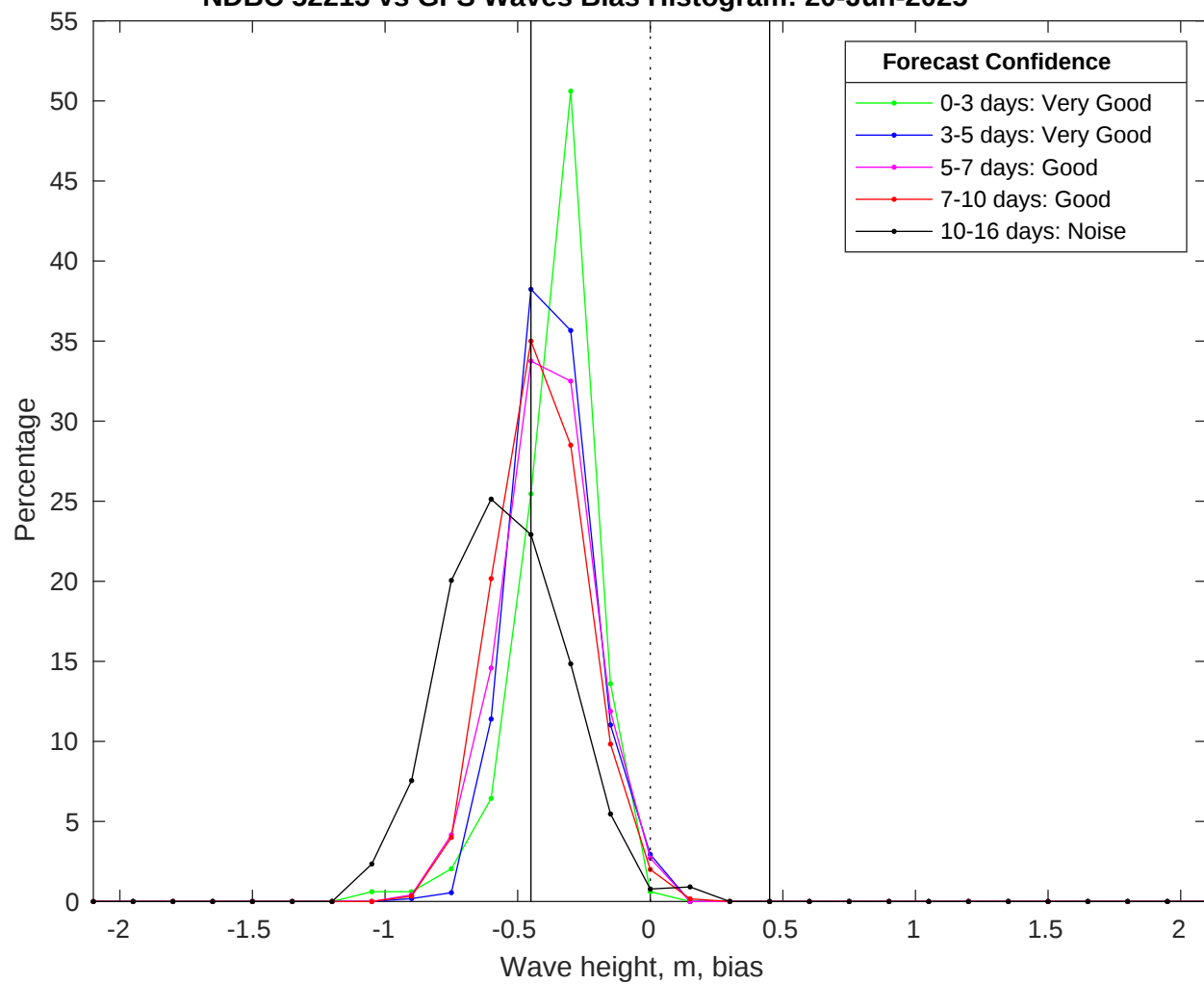
NDBC 52213 vs GFS Waves Bias Histogram: 20-Jun-2025
