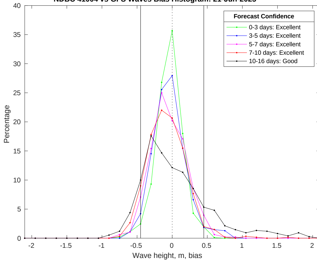
NDBC 41004 vs GFS Waves Bias Histogram: 21-Jun-2025
