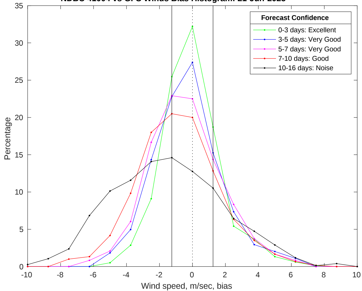
NDBC 41004 vs GFS Winds Bias Histogram: 21-Jun-2025
