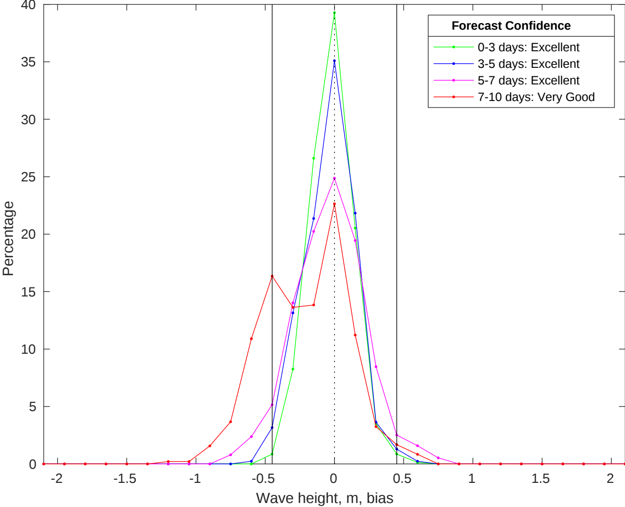
NDBC 41013 vs CMEMS Waves Bias Histogram: 21-Jun-2025
