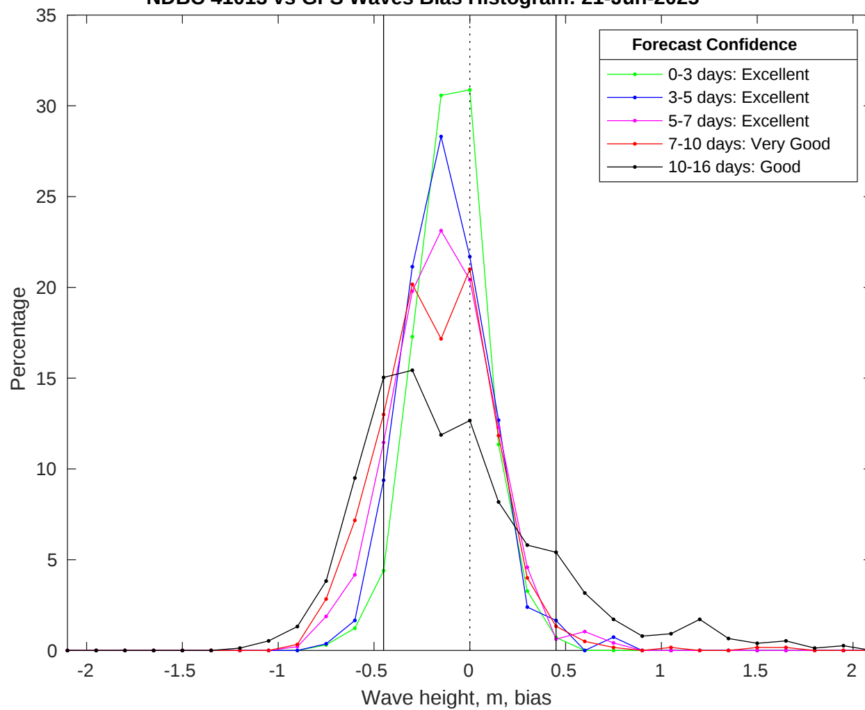
NDBC 41013 vs GFS Waves Bias Histogram: 21-Jun-2025
