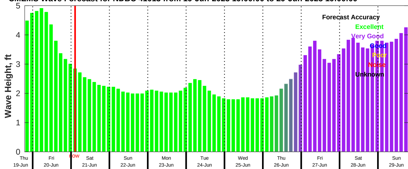
CMEMS Wave Forecast for NDBC 41013 from 19-Jun-2025 19:00:00 to 29-Jun-2025 19:00:00
