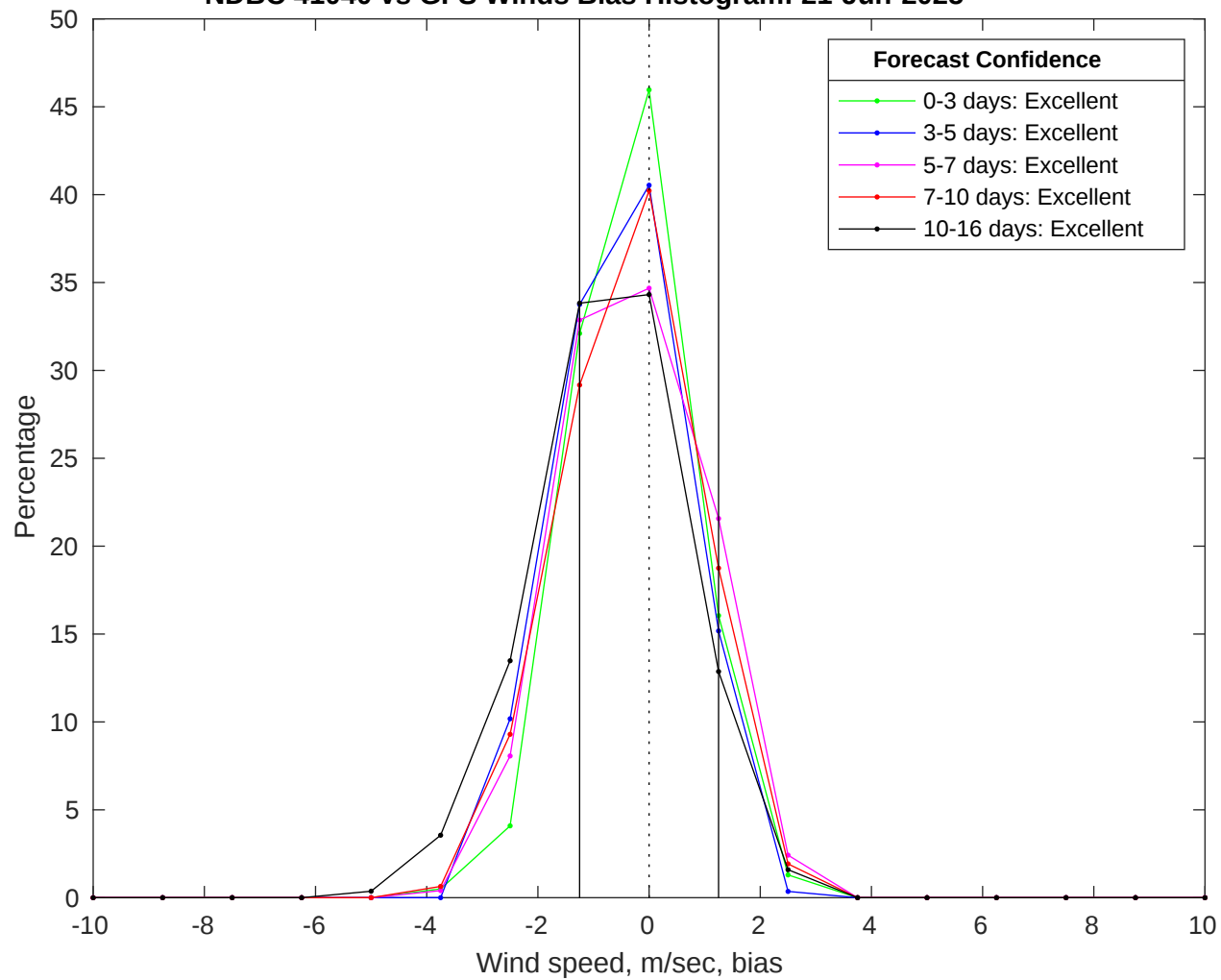
NDBC 41040 vs GFS Winds Bias Histogram: 21-Jun-2025
