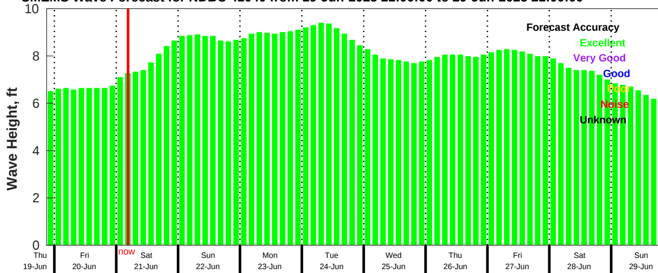
CMEMS Wave Forecast for NDBC 41040 from 19-Jun-2025 21:00:00 to 29-Jun-2025 21:00:00
