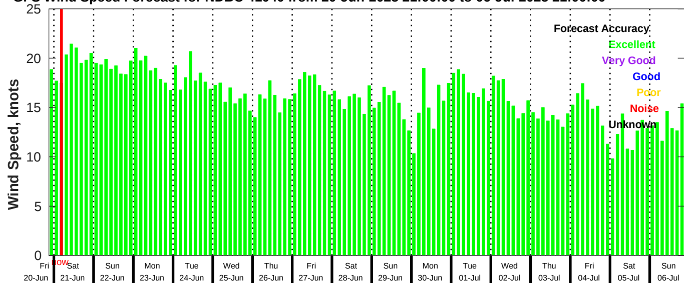
GFS Wind Speed Forecast for NDBC 41040 from 20-Jun-2025 21:00:00 to 06-Jul-2025 21:00:00
