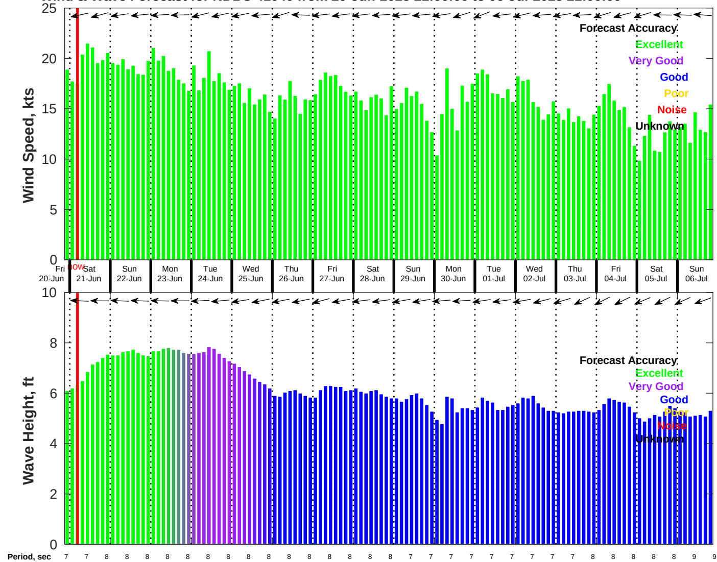
Wind & Wave Forecast for NDBC 41040 from 20-Jun-2025 21:00:00 to 06-Jul-2025 21:00:00
