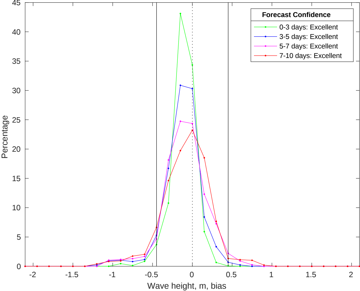
NDBC 42019 vs CMEMS Waves Bias Histogram: 21-Jun-2025
