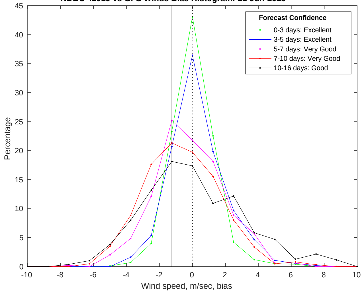
NDBC 42019 vs GFS Winds Bias Histogram: 21-Jun-2025
