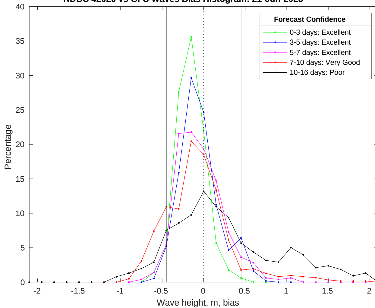
NDBC 42020 vs GFS Waves Bias Histogram: 21-Jun-2025
