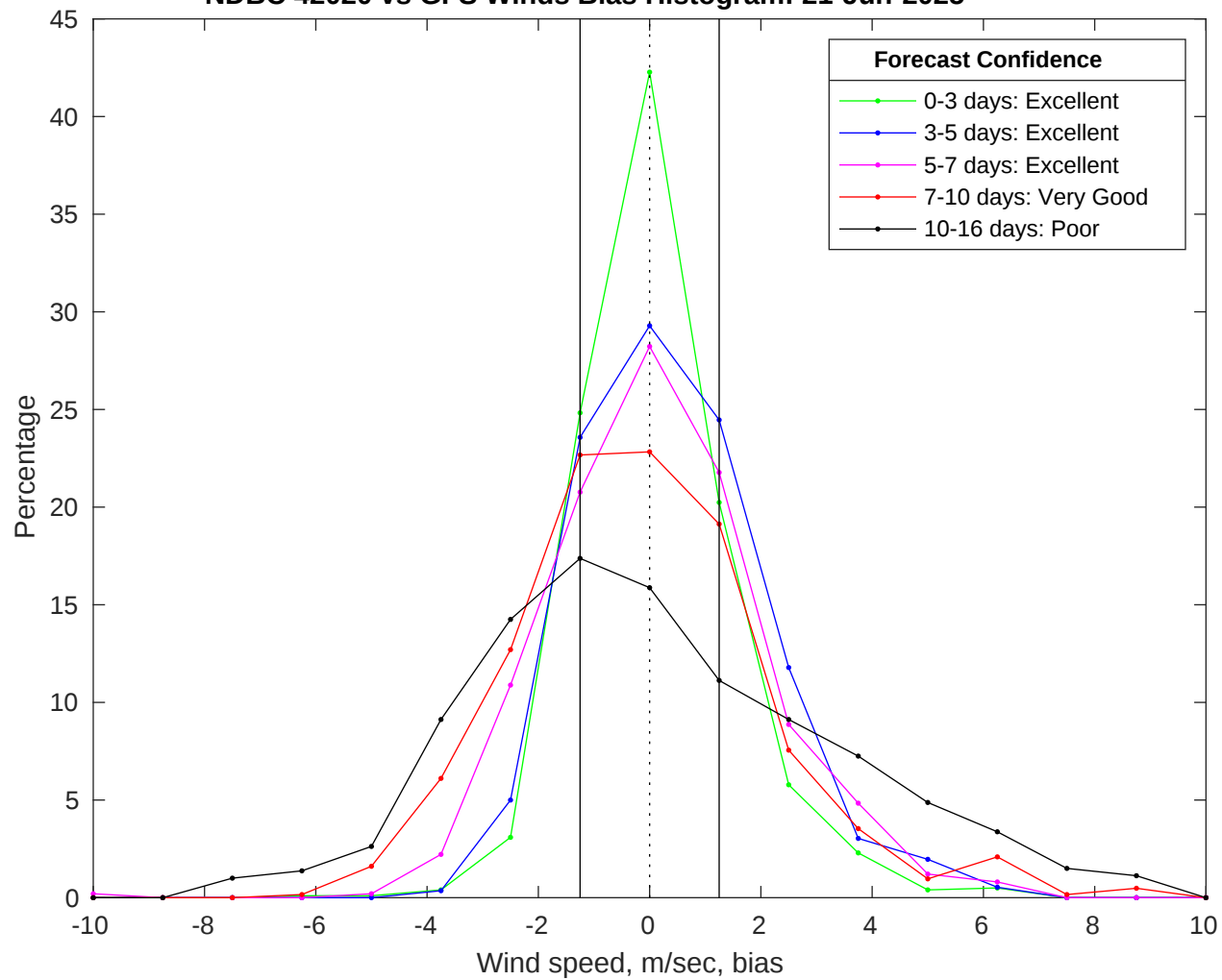
NDBC 42020 vs GFS Winds Bias Histogram: 21-Jun-2025
