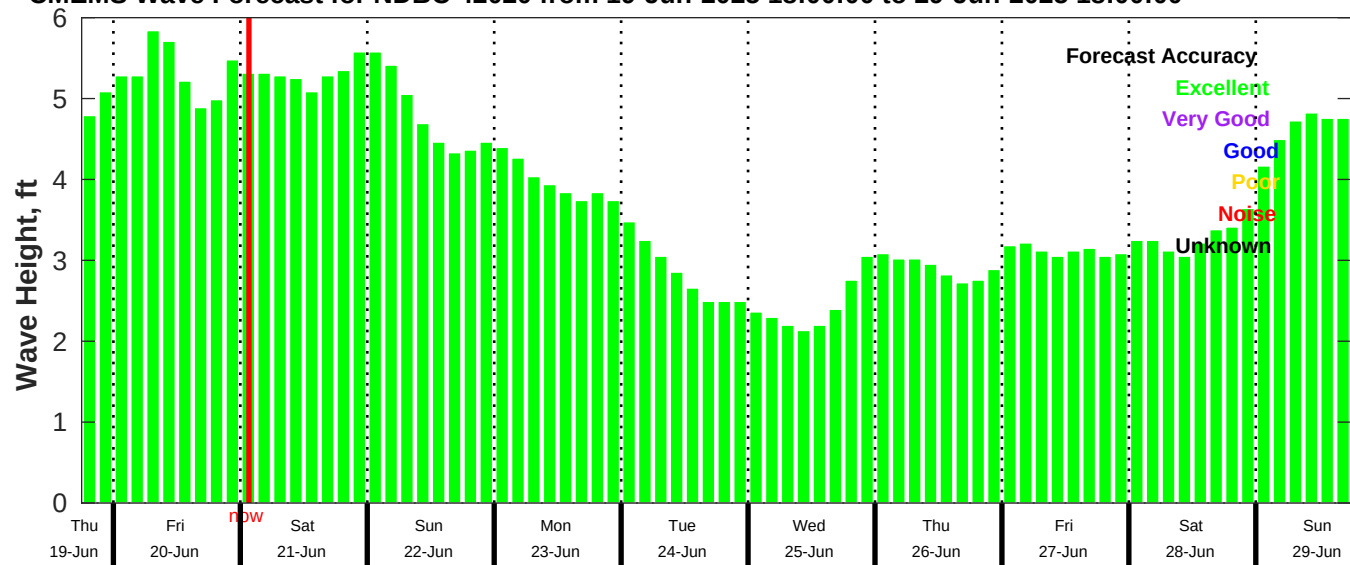
CMEMS Wave Forecast for NDBC 42020 from 19-Jun-2025 18:00:00 to 29-Jun-2025 18:00:00
