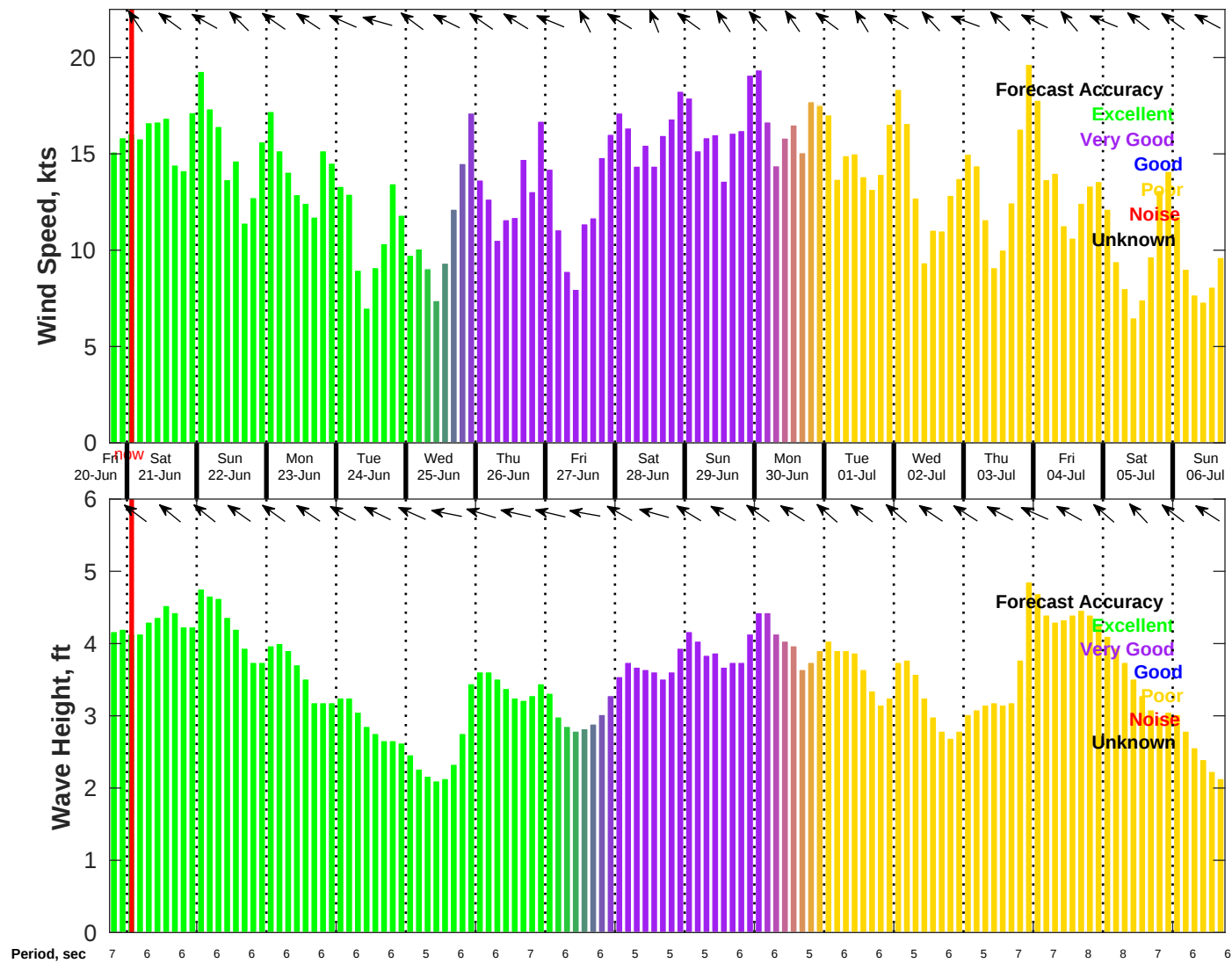
Wind & Wave Forecast for NDBC 42020 from 20-Jun-2025 18:00:00 to 06-Jul-2025 18:00:00
