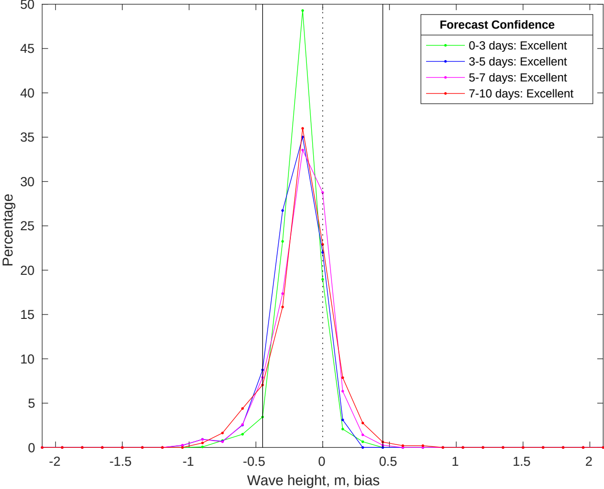
NDBC 42035 vs CMEMS Waves Bias Histogram: 21-Jun-2025
