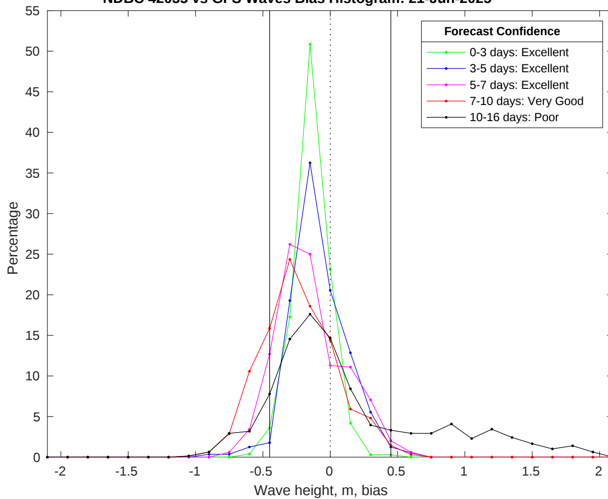
NDBC 42035 vs GFS Waves Bias Histogram: 21-Jun-2025
