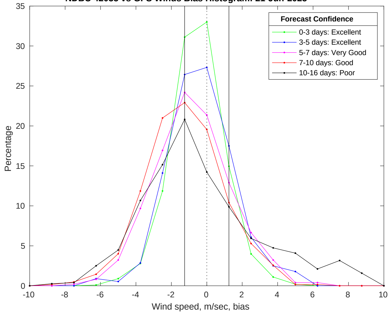
NDBC 42035 vs GFS Winds Bias Histogram: 21-Jun-2025
