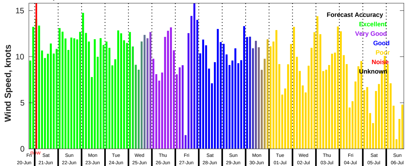
GFS Wind Speed Forecast for NDBC 42035 from 20-Jun-2025 18:00:00 to 06-Jul-2025 18:00:00
