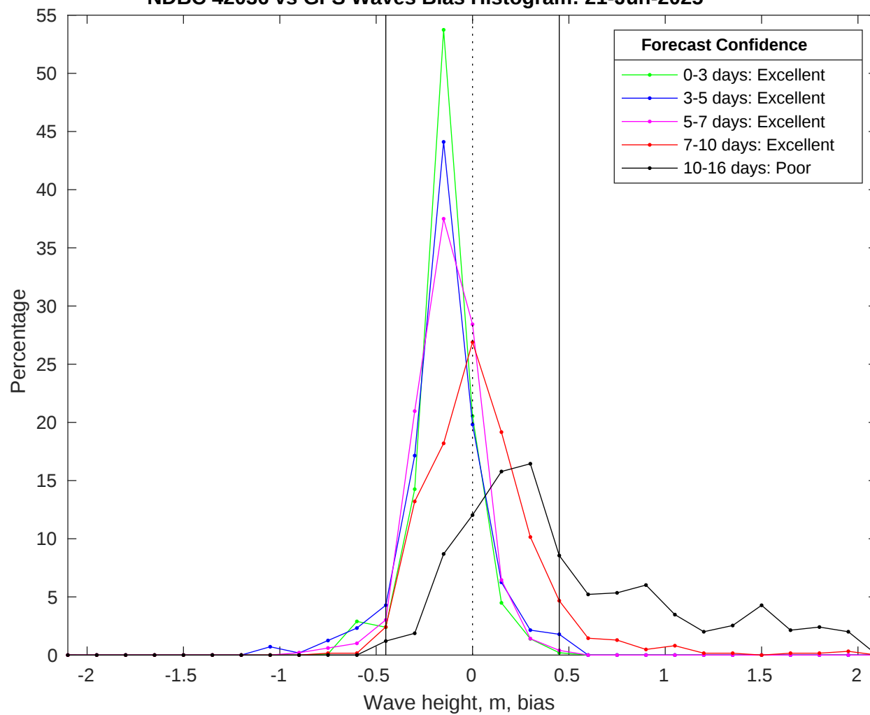
NDBC 42036 vs GFS Waves Bias Histogram: 21-Jun-2025
