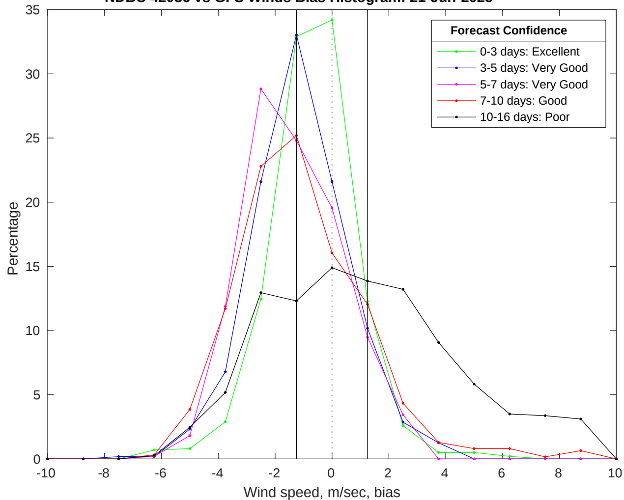
NDBC 42036 vs GFS Winds Bias Histogram: 21-Jun-2025
