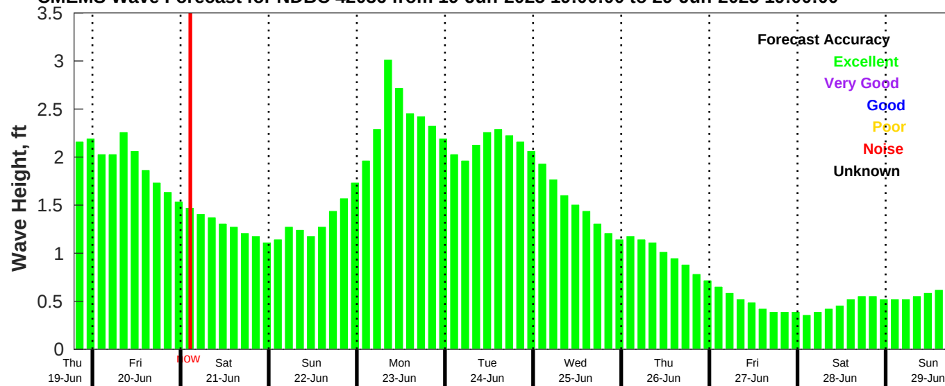
CMEMS Wave Forecast for NDBC 42036 from 19-Jun-2025 19:00:00 to 29-Jun-2025 19:00:00
