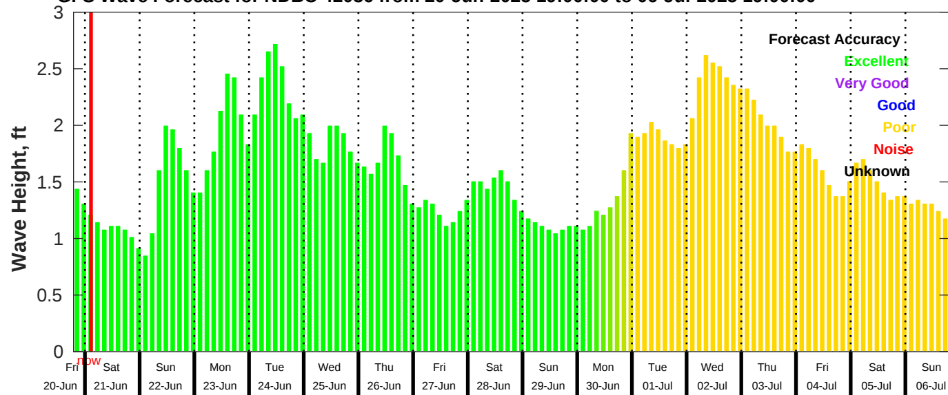
GFS Wave Forecast for NDBC 42036 from 20-Jun-2025 19:00:00 to 06-Jul-2025 19:00:00
