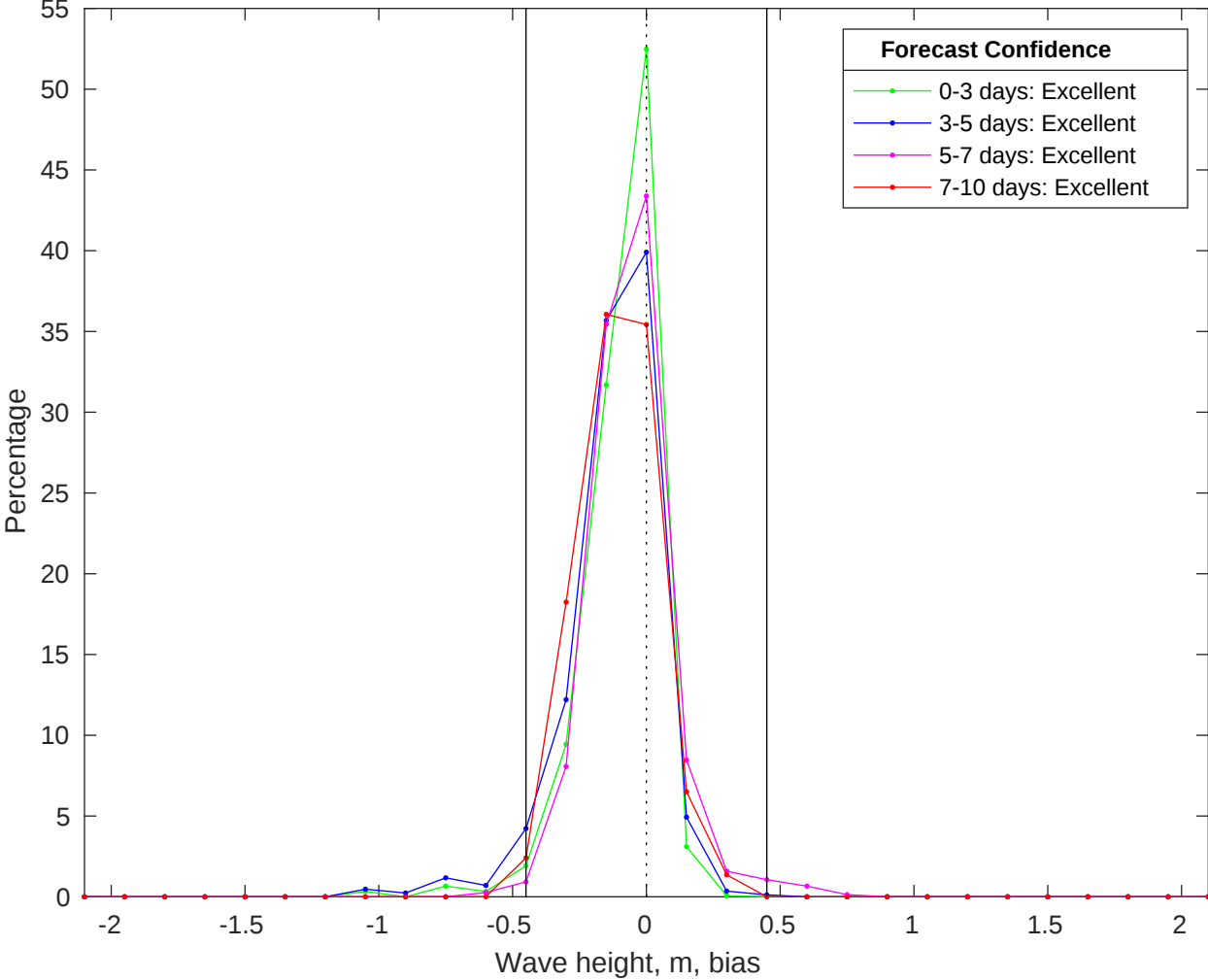
NDBC 42040 vs CMEMS Waves Bias Histogram: 21-Jun-2025
