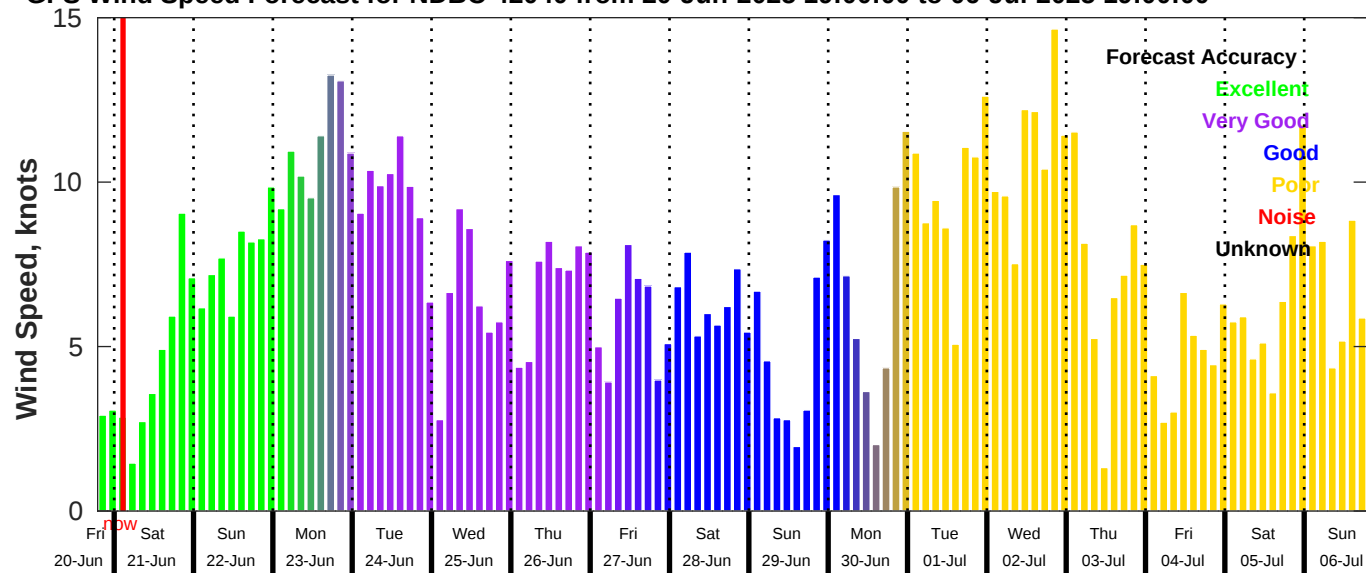
GFS Wind Speed Forecast for NDBC 42040 from 20-Jun-2025 19:00:00 to 06-Jul-2025 19:00:00
