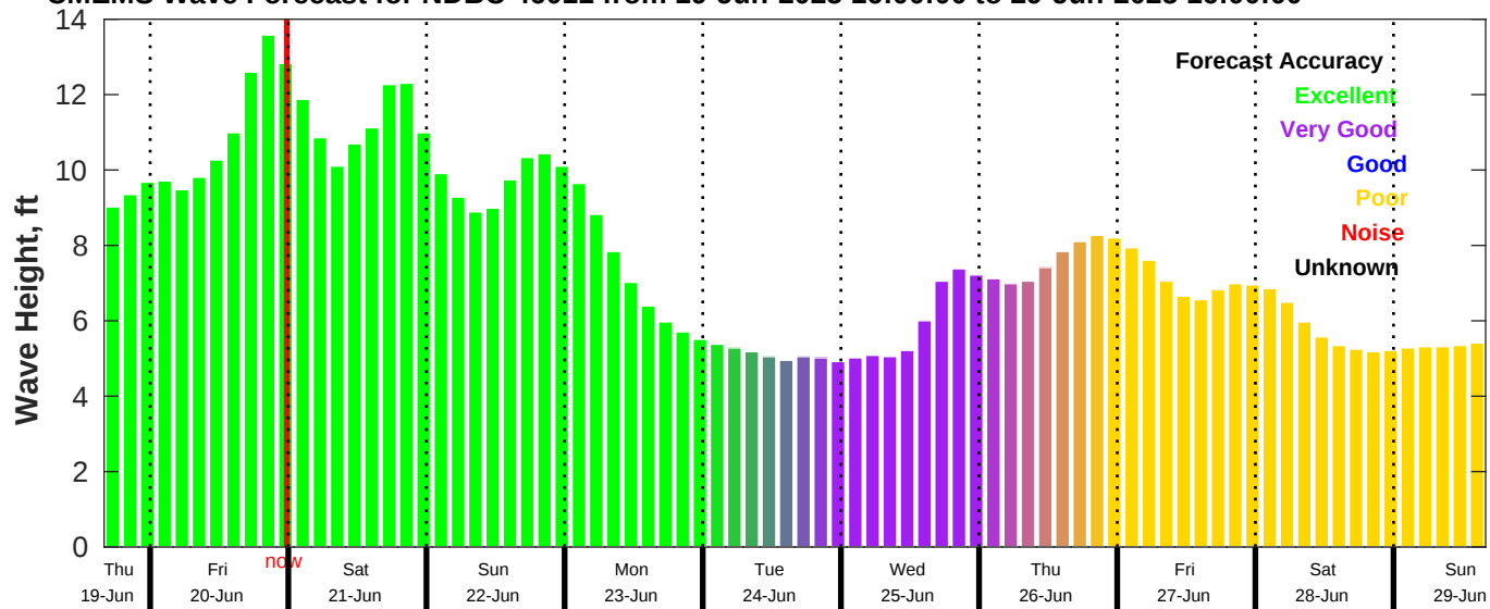
CMEMS Wave Forecast for NDBC 46011 from 19-Jun-2025 16:00:00 to 29-Jun-2025 16:00:00
