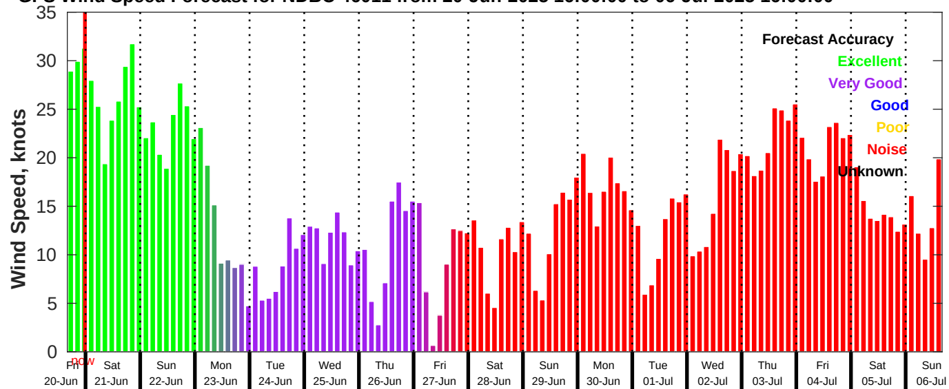
GFS Wind Speed Forecast for NDBC 46011 from 20-Jun-2025 16:00:00 to 06-Jul-2025 16:00:00
