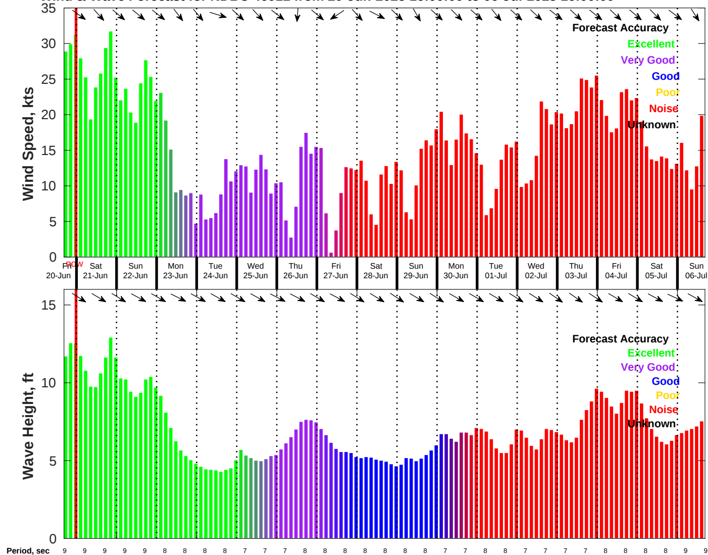
Wind & Wave Forecast for NDBC 46011 from 20-Jun-2025 16:00:00 to 06-Jul-2025 16:00:00
