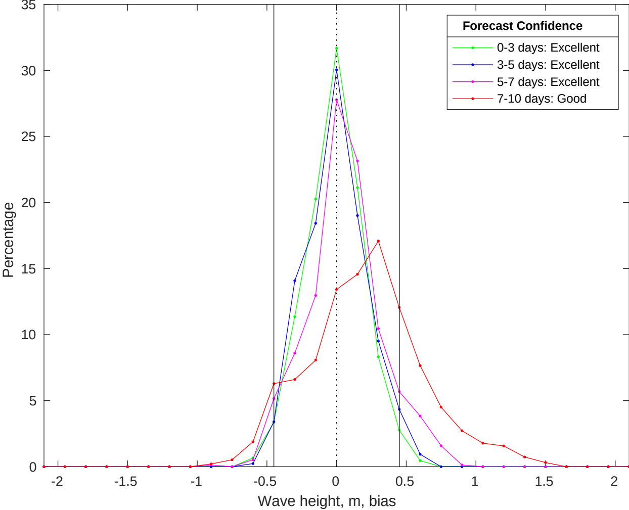
NDBC 46028 vs CMEMS Waves Bias Histogram: 21-Jun-2025
