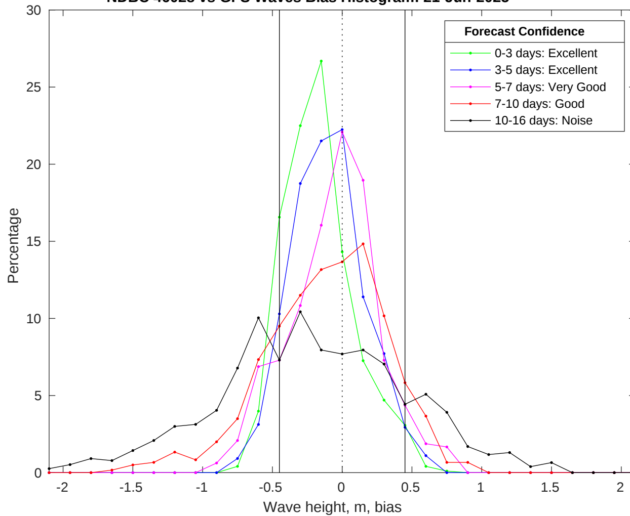
NDBC 46028 vs GFS Waves Bias Histogram: 21-Jun-2025
